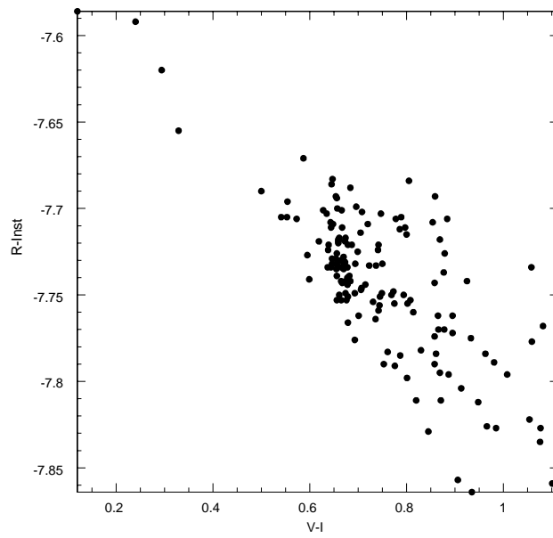
Figure 4. R-magnitude residuals vs. color for a KAF0400E CCD.
