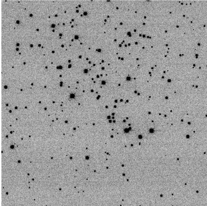
Figure 1. CCDV image of M67, north up and east left. Field of view is 11 x 11 arcmin.
