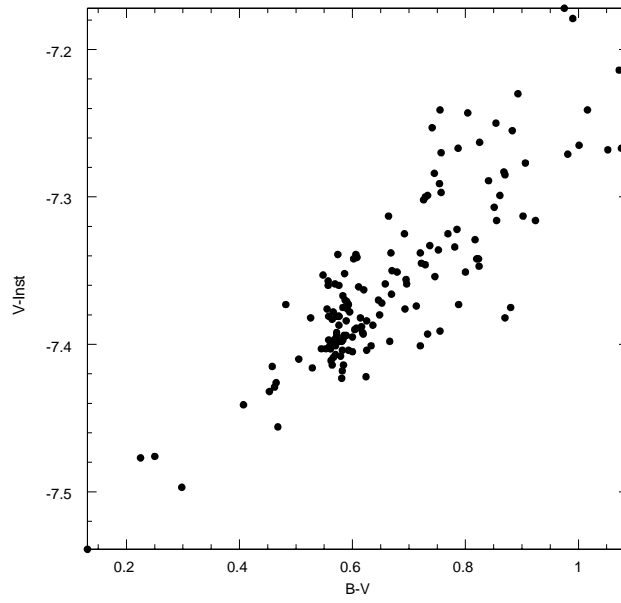
Figure 3. V-magnitude residuals vs. color for a KAF0400E CCD.
