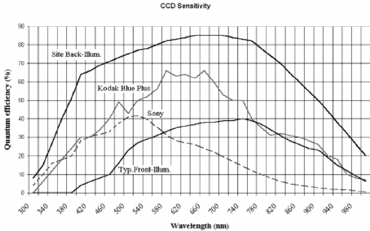
Figure 2. Sensitivity vs. wavelength curve for various CCD types (Apogee, Inc.; Brown 2000).
