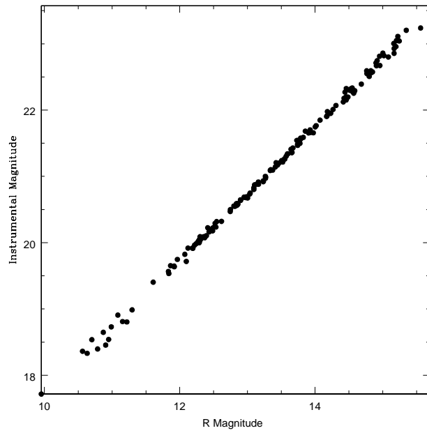
Figure 5. Instrumental unfiltered KAF0400E magnitude vs. Cousins R-magnitude for M67.
