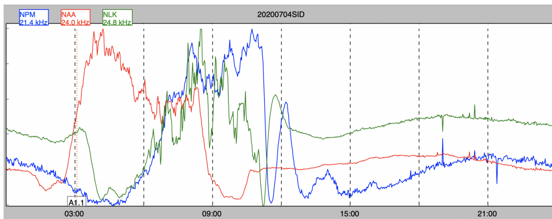
Figure 2: VLF recording at Fort Collins, Colorado.
