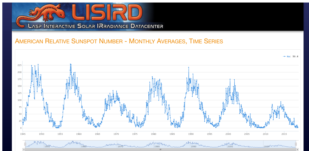
Figure 1: LASP has a new web site, Lasp Interactive Solar IRadiance Datacenter (LISIRD) which houses solar data from many observatories. And now they display the AAVSO daily and monthly R_a back to 1944. ( http://lasp.colorado.edu/lisird/ )
