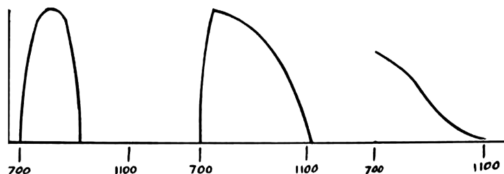
Figure 1. Low-budget sketch of (l-r) Cousins I, RG9, and CCD (KAF-16803) response curves.
