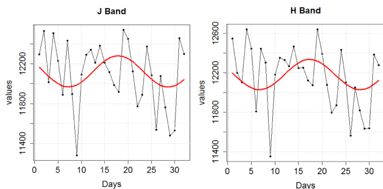
Figure 5. J- and H-band period plots
