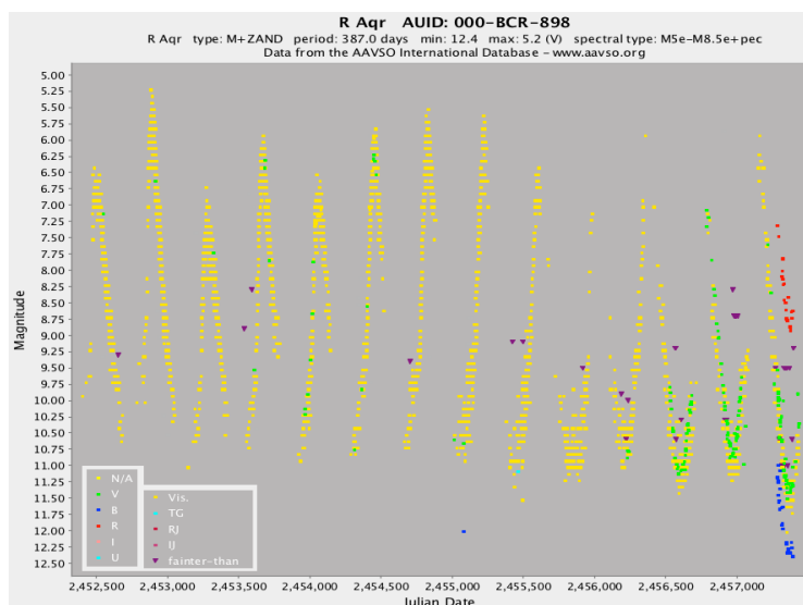
Figure 2: AAVSO light curve of the symbiotic Mira R Aqr JD 2452388–2457417 (19 April 2002–29 January 2016). 202 observers worldwide contributed 3,134 visual and multicolor observations to this light curve.
