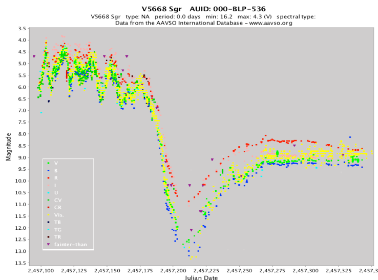
Figure 1. AAVSO multicolor light curve of V5668 Sgr, March–November 2015 (JD 2457095–2457350). 128 observers worldwide contributed 3,809 observations to this light curve.
