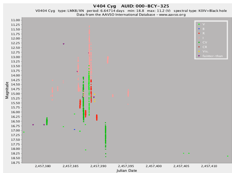
Figure 4: AAVSO light curve of the X-ray black hole binary V404 Cyg JD 2457376–2457413 (19 December 2015–26 January 2016). 18 observers contributed 1,034 visual and multicolor observations to this light curve.
