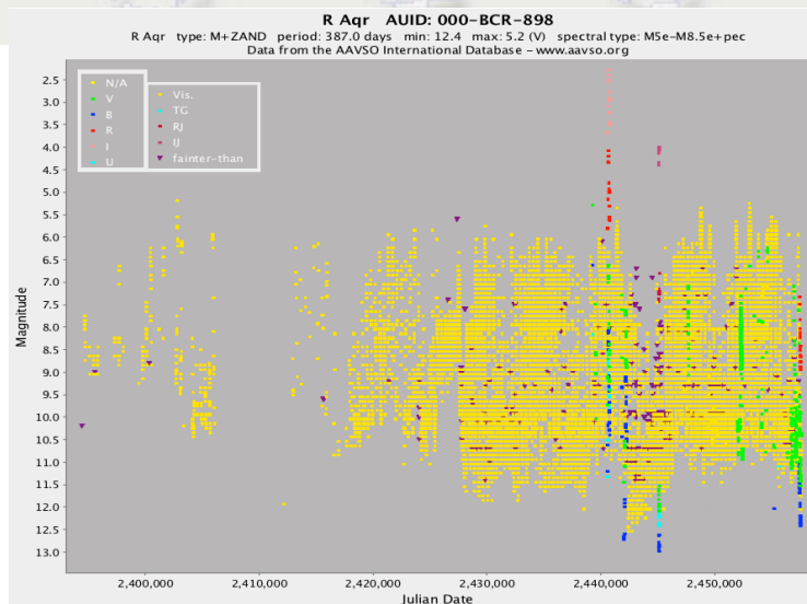
Figure 1: AAVSO historical light curve of the symbiotic Mira R Aqr JD 2394441–2457417 (28 August 1843–29 January 2016). 959 observers worldwide contributed 20,380 visual and multicolor observations to this light curve.
