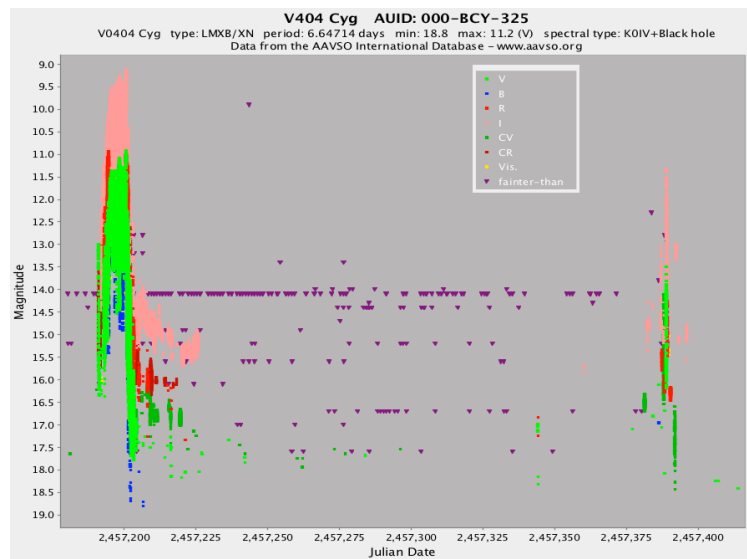
Figure 3: AAVSO light curve of the X-ray black hole binary V404 Cyg JD 2457180–2457413 (6 June 2015–26 January 2016). 82 observers contributed 71,447 visual and multicolor observations to this light curve.
