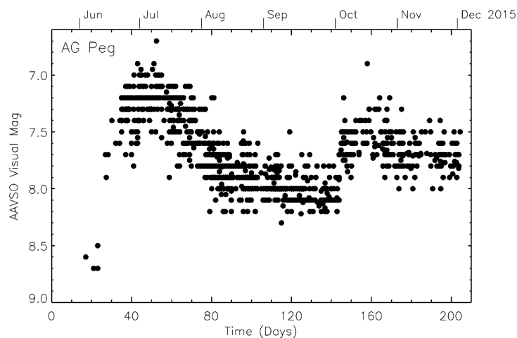
Figure 2. AAVSO visual observations of AG Peg for the first 200 days post-outburst. 87 visual observers worldwide contributed 1,189 observations to this light curve.
