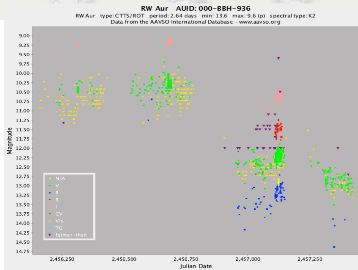
Figure 6. AAVSO light curve of the T Tauri star RW Aur JD 2456156–2457422 (16 August 2012–3 February 2016). 75 observers contributed 2,894 visual and multicolor observations to this light curve.
