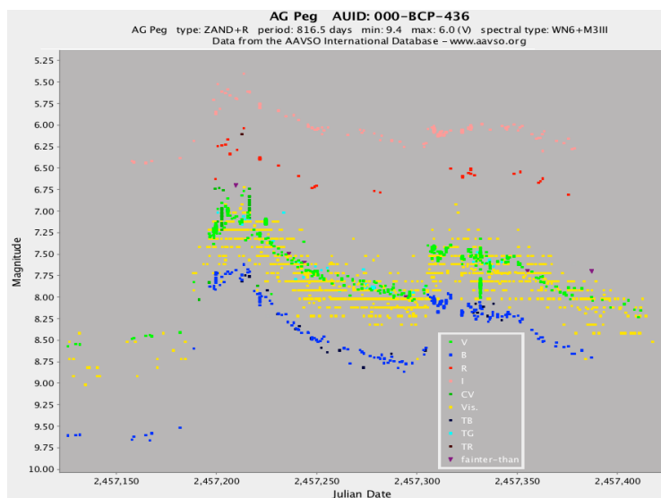
Figure 1. AAVSO multicolor light curve of AG Peg, April 2013-January 2016. 123 observers worldwide contributed 2,608 observations to this light curve.
