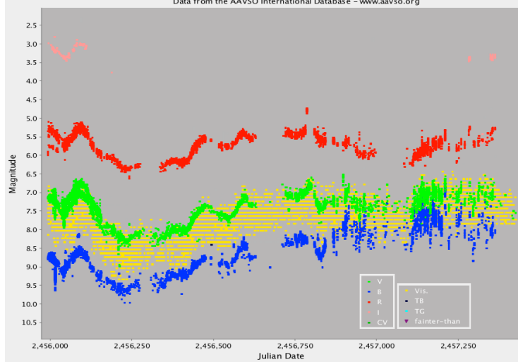
Figure 5: AAVSO light curve of the symbiotic star CH Cyg JD 2455988–2457420 (1 March 2012–1 February 2016). 228 observers contributed 27,400 visual and multicolor observations to this light curve.
