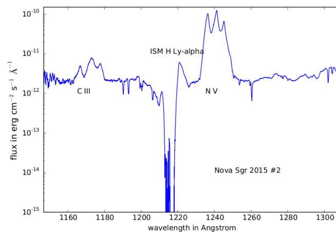
Figure 2. HST STIS spectrum of V5668 Sgr, region around Hydrogen Lyman-alpha line.
