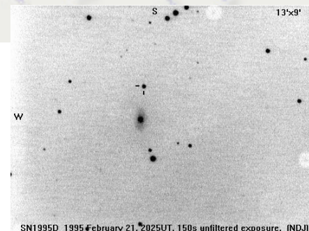
SN1995D 1995 February 21, 2025UT, 150s unfiltered exposure. (NDJ) SN1995D in NGC 2962
