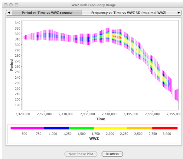
WWZ contour plot of T Umi
