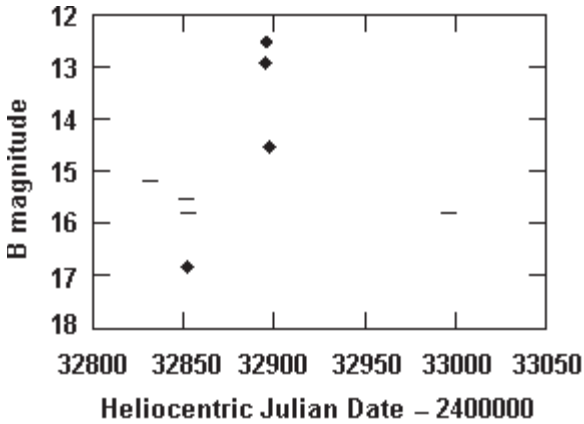
Figure 2. The light curve around the 1948 outburst. Diamonds represent observed magnitude; lines represent brightness upper limit (fainter-than).
