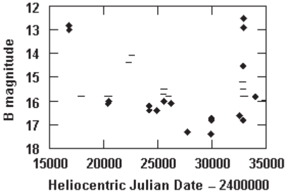
Figure 1. The light curve for Ross 4 from 1904 to 1952. Diamonds represent observed magnitude; lines represent brightness upper limit (fainter-than).
