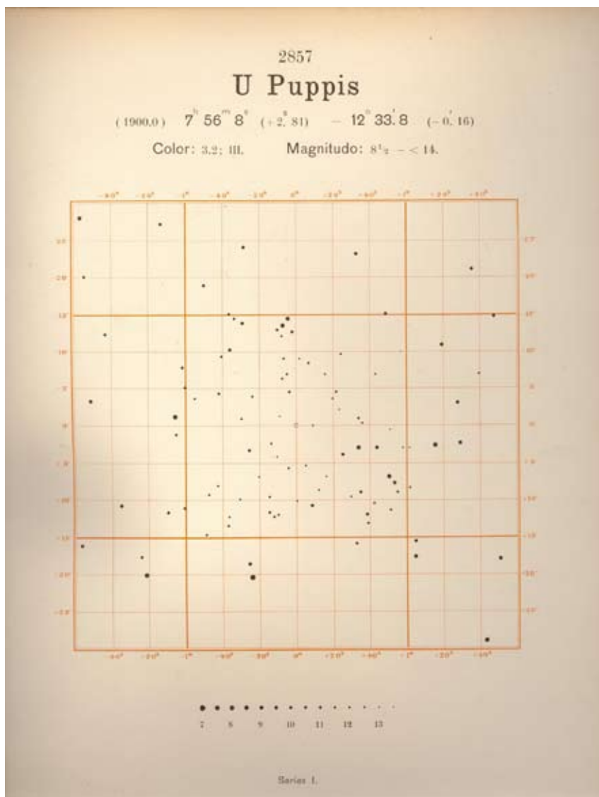
Figure 1. Chart for U Pup from Atlas Stellarum Variabilium , Series I (Hagen 1899).
