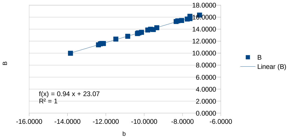
Linearity Check Standard B vs instrumental b
