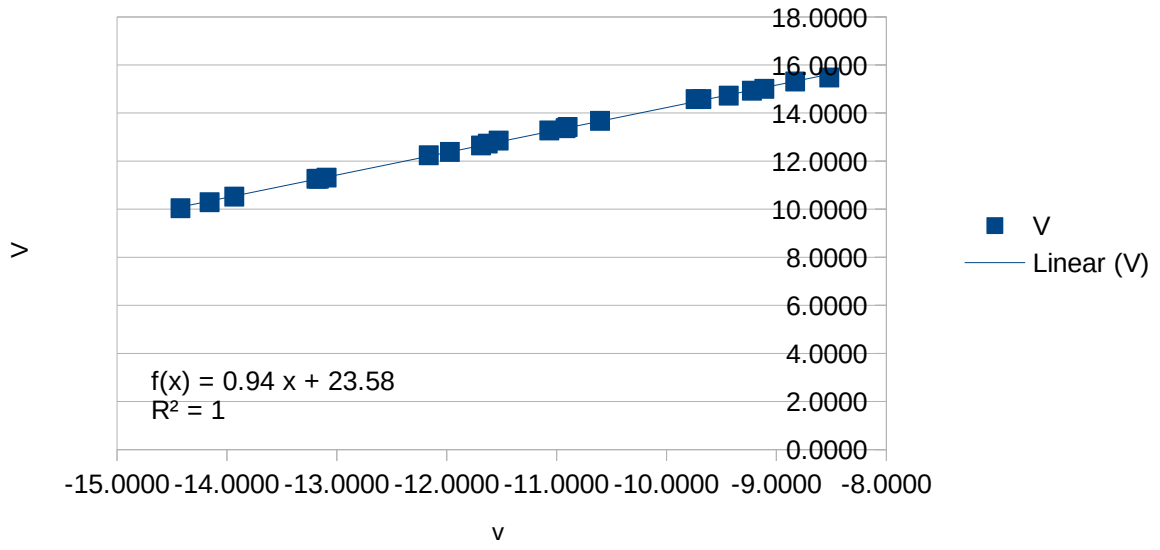
Linearity check Standard V vs instrumental v
