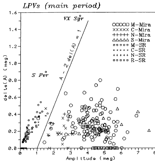
Figure 1. Amplitude A versus amplitude instability \delta_A for the main period of LPVs. The line is the cutoff between Mira and SR, given by A - 2\delta_A = 1 .
