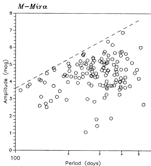
Figure 5. Period P versus amplitude A for M -Miras, showing the upper limit as a function of period.
