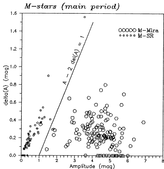
Figure 3. Amplitude A versus amplitude instability \delta_A , for the main period of M -type LPVs.
