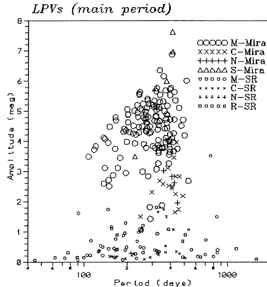
Figure 2. Period P versus amplitude A for the main period of LPVs.
